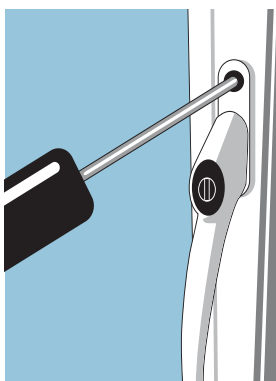
Figure 76. Tighten top fixing using Phillips screwdriver and push cover cap back into place.
